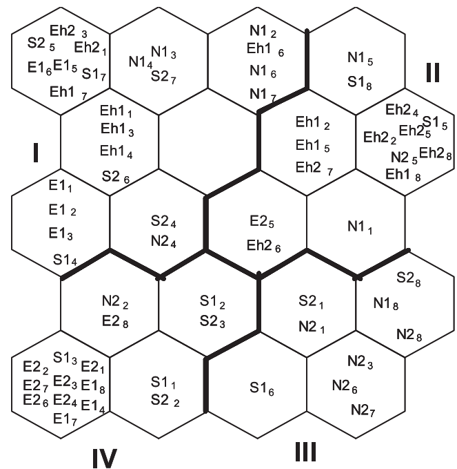
Fig. 2. Classification of samples using presence-absence data through the learning process of the self-organizing map. S: Soumié River, E: Eholié River, Eh: Ehania River; N: Noé River; 1: upstream, 2: downstream. Index 1 to 8 = number of samples.
